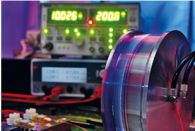
Image 3: Laboratory setup of the thulium-doped fiber amplifier for the Einstein Telescope. © Fraunhofer ILT, Aachen.
