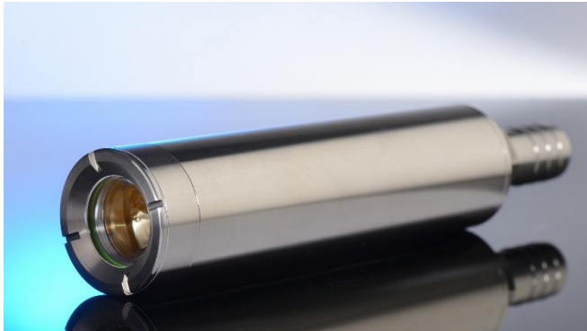
Image 1: The 2D fluorescence probe developed at the Fraunhofer ILT is a central building block for inline water and wastewater monitoring. © Fraunhofer ILT, Aachen, Germany.
